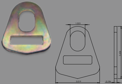
DR-2-16M 2" DELTA RING – 16,200 LB.
