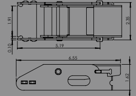
512 2" OVERCENTER BUCKLE - 5,000 LB.
