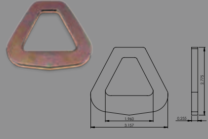
DR-2-10M 2" DELTA RING – 10,000 LB.
