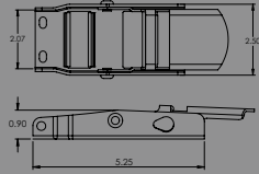
504 2" OVERCENTER BUCKLE
