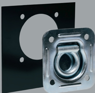
4275 SQUARE RECESSED FLOOR RING, ROUND MOUNTING HOLES, ZINC 4275-MP UNDER FLOOR MOUNTING PLATE FOR 4275 4277-MP-K
