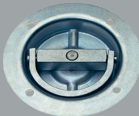
4280 ROUND RECESSED FLOOR RING 360°, ZINC
